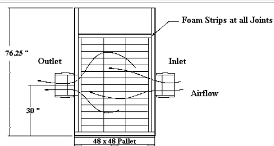
Section View Note: All dimensions are in inches
