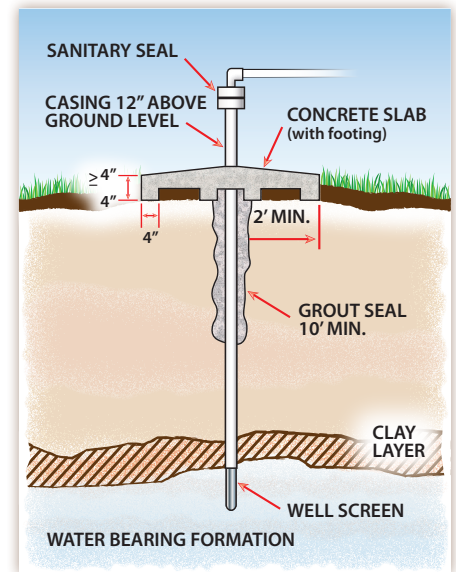
▲ Diagram showing proper drilled well construction. Notice the concrete slab around the wellhead that prevents surface water from moving down the outside of the well casing. This type of slab is critical for both drilled and bored wells to prevent contamination.
