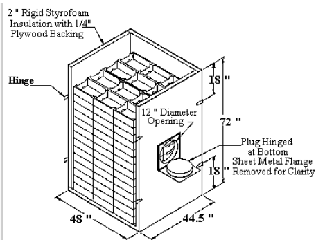
Pictorial View Top and One Side Removed for Clarity
